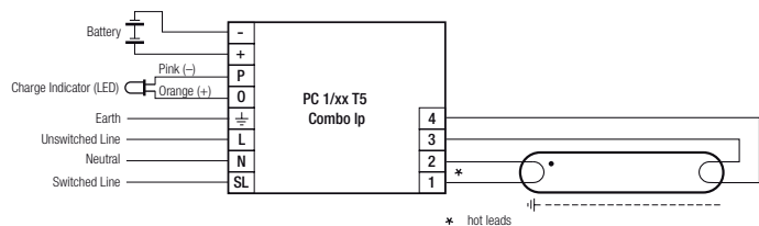
Wiring diagram PC T5 COMBO Ip with single T5 lamp
