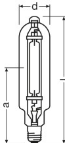
Product line drawing with letters HQI-T 2000 W/N/E SUPER E40 | HQI-T 2000 W/N/SN SUPER E40 | HQI-T 2000 W/N 230V E40 | HQI-T 2000 W/D E40 | HQI-T 2000 W/N E40 | HQI-T 2000 W/D/I E40
