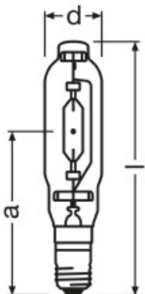
Product line drawing with letters HQI-T 1000 W/D E40 | HQI-T 1000 W/N E40
