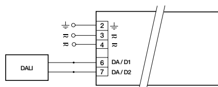
DALI PCA T5 EXCEL one4all
