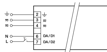
switchDIM PCA T5 EXCEL one4all
