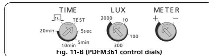
Fig. 11-B (PDFM361 control dials)
